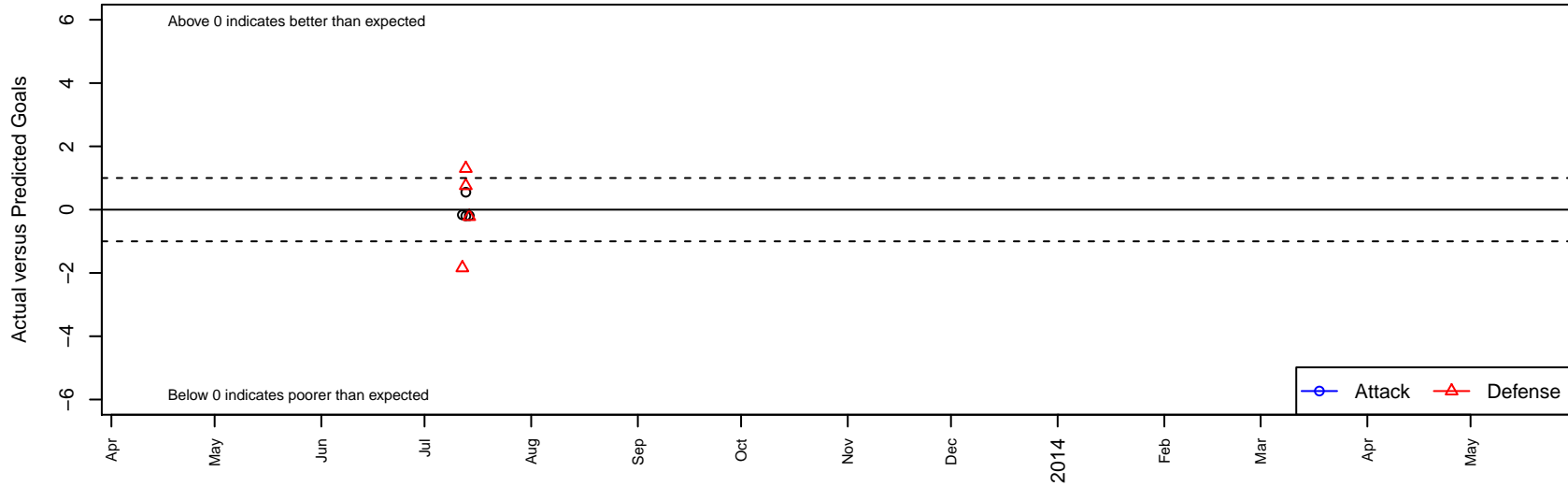
NEU Ajax Silver B00 Dots are actual minus expected GF (blue circles) and GA (red triangles). Blue line is smoothed change in attack strength. Red is smoothed change in defense strength.
